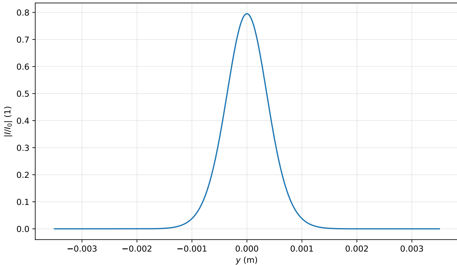
Intensity profile I(x=0, y, z=1.513)/I_0 , P_{in}=0.3P_{cr} , artificial time
